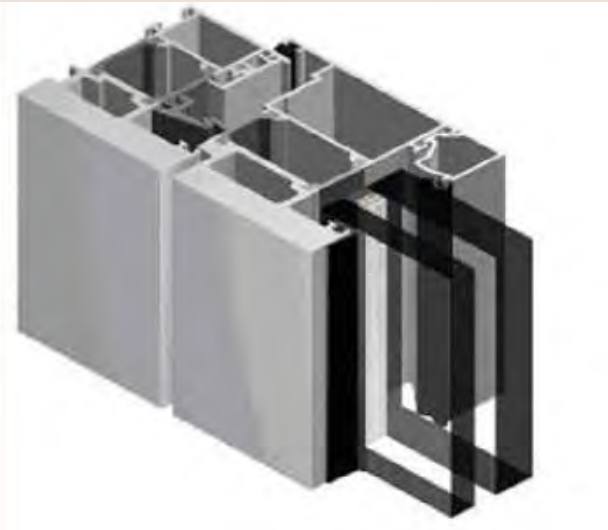
Figure 35: Bullet-resistant window and door construction
