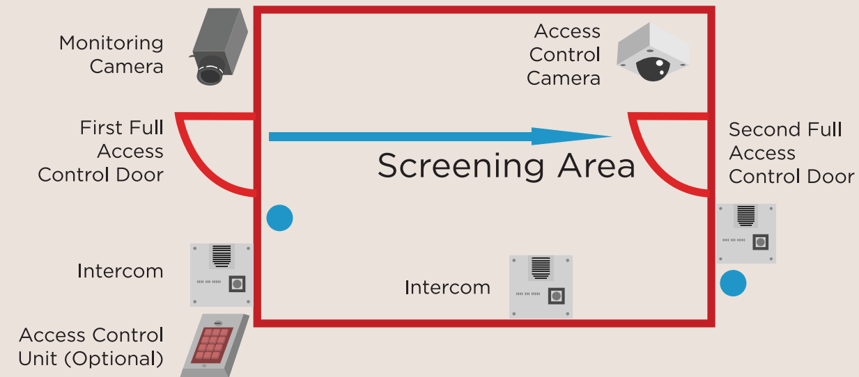
Figure 15: Typical interlocking system entry point
