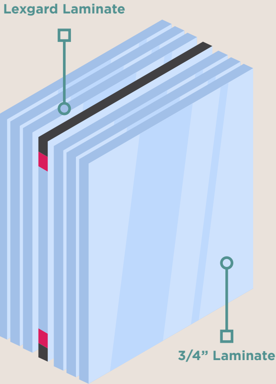
Figure 40: Bullet and blast resistant glazing system
