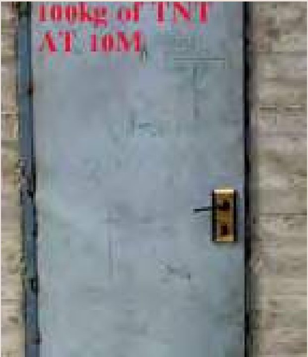
Figure 43: Blast resistant door after a 100kg explosion at 10m
